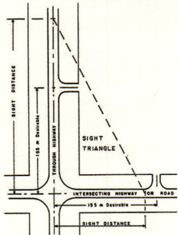
FIGURE 3. SIGHT TRIANGLE DIAGRAM
