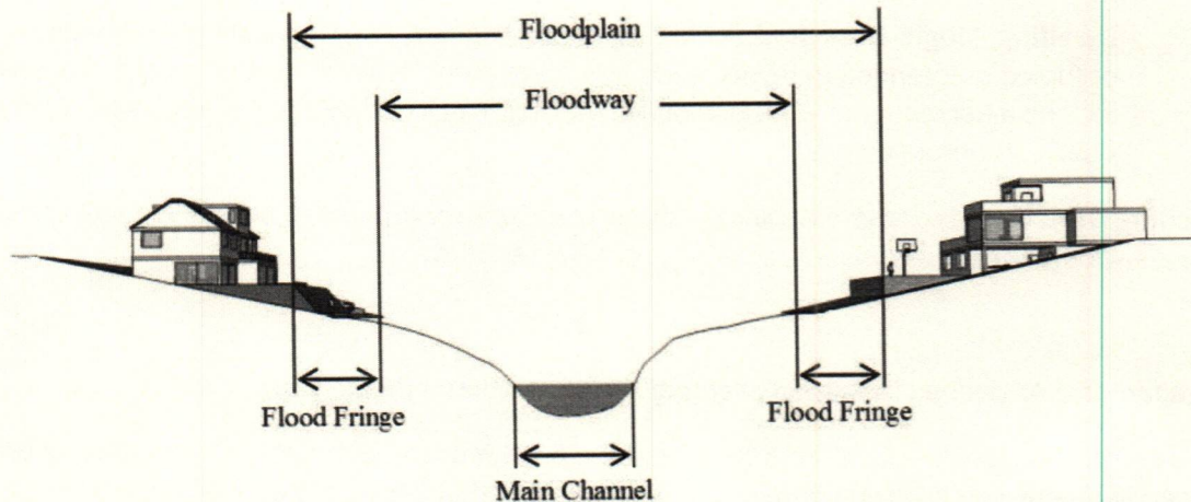
FIGURE 5: CROSS-SECTION OF A FLOOD FRINGE AND FLOODPLAIN
